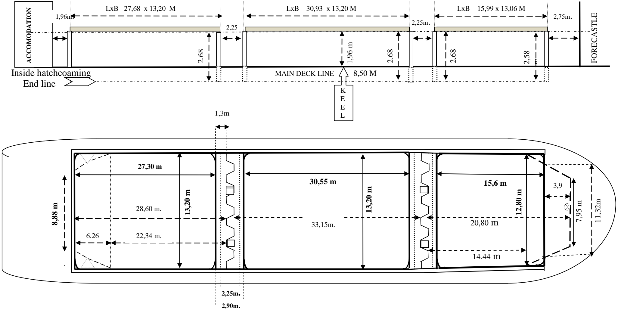
HATCHES (HATCH-COAMINGS) FROM ABOVE VIEW
